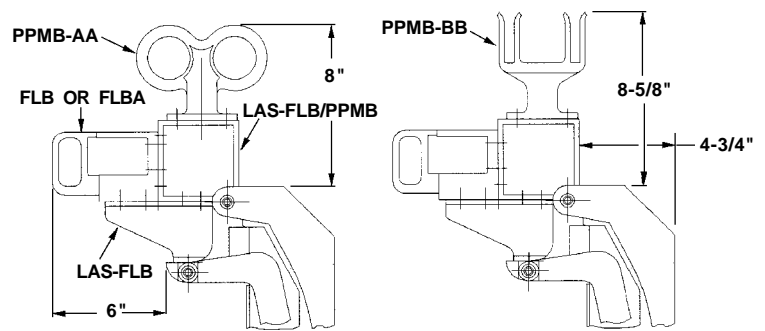
FIGURE 18. MODEL LAS-FLB/PPMB EXTRUSION ADDED TO SUPPORT PPMB-AA (DOUBLE RING) OR PPMB-BB (DOUBLE FORK) PIKE POLE MOUNTING BRACKET
