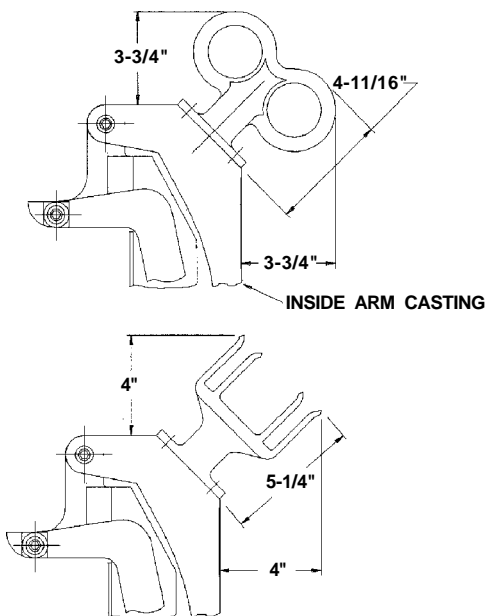
FIGURE 19. MODEL PPMB-AA (DOUBLE RING) OR PPMB-BB (DOUBLE FORK) PIKE POLE MOUNTING BRACKETS MAY BE ATTACHED DIRECTLY TO THE INSIDE ARM CASTING (3097-105-102)
