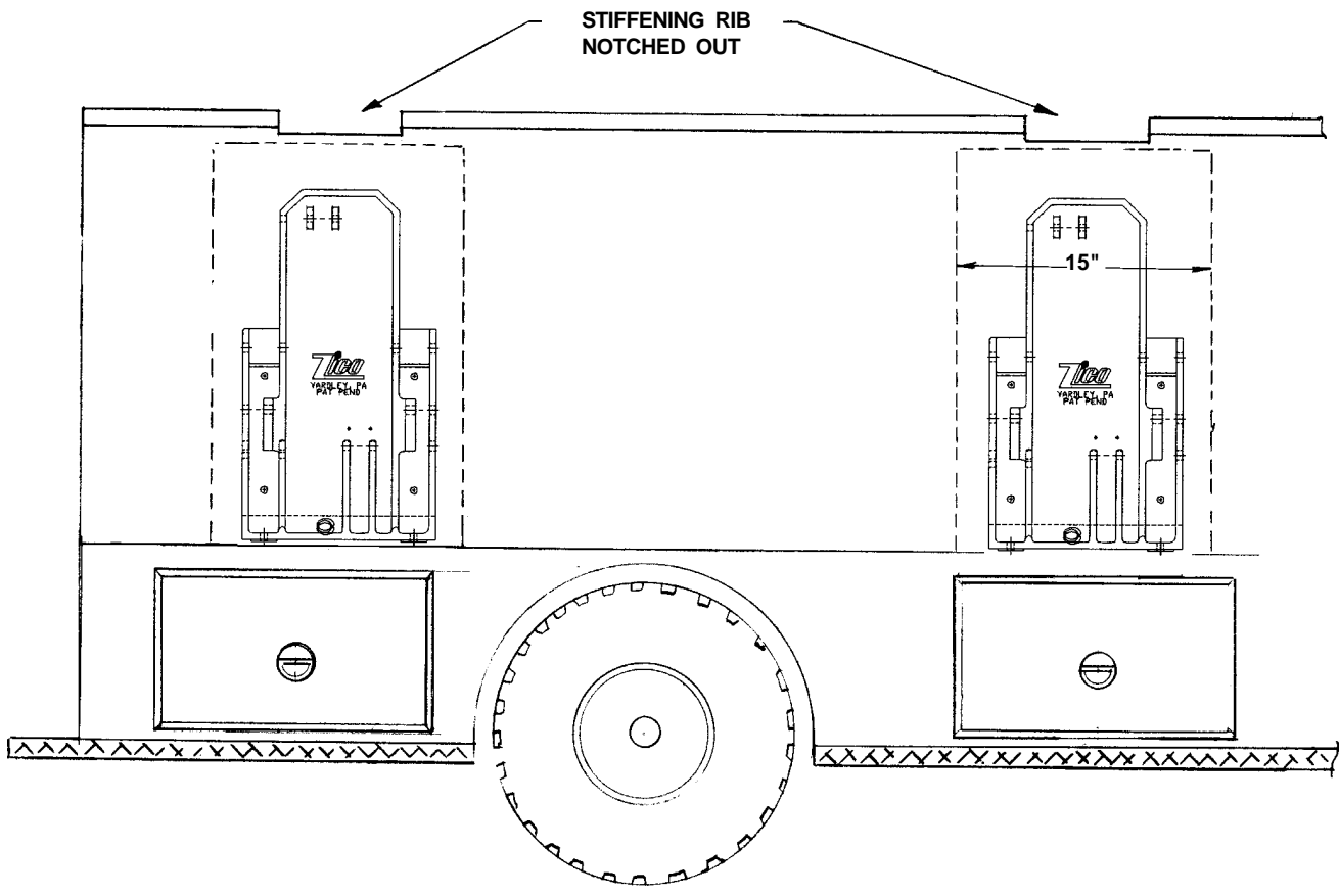
FIGURE 7. COMMON INSTALLATION USING STIFFENING/BACKING PLATE
