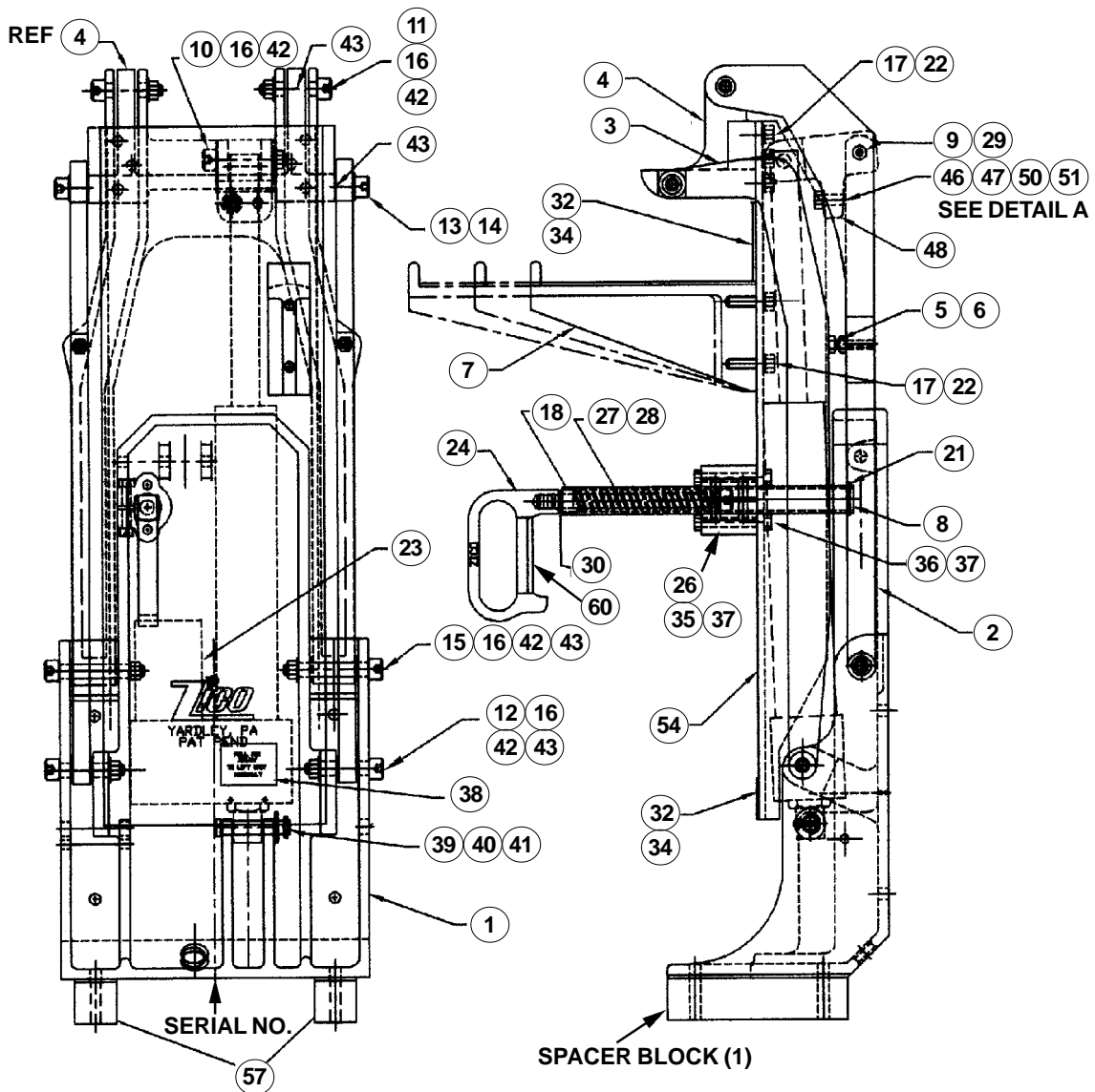
FIGURE 3. MODEL LAS-____ STANDARD MODEL SHOWN WITH OPTIONAL SPACER BLOCKS UNDER BASE CASTING
