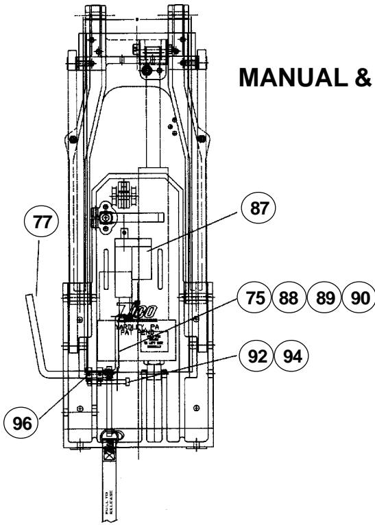
FIGURE 25. LOCKING SYSTEM COMPONENTS
