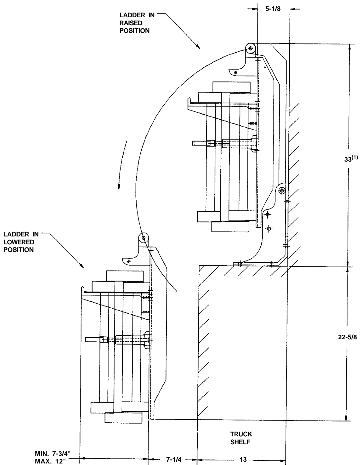
FIGURE 5. SIDE VIEW MODEL LAS-_____
