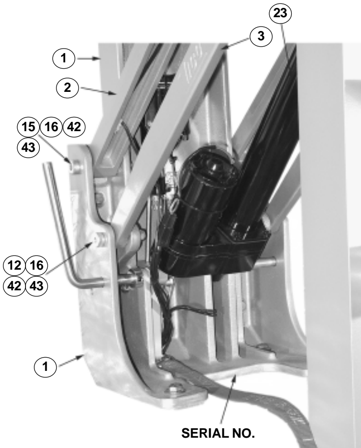
FIGURE 31. LAS-___ COMPONENTS See Chart 1 Parts List Page 14 and Figure 3 Drawings Page 15
