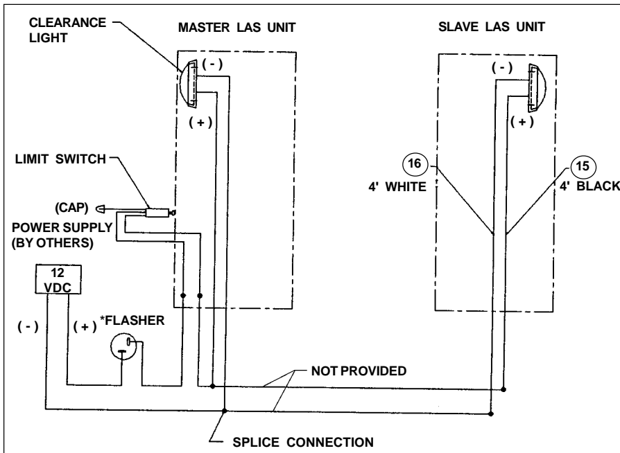
FIGURE 20. FLASHING LIGHT KIT MODEL LAS-FLK
