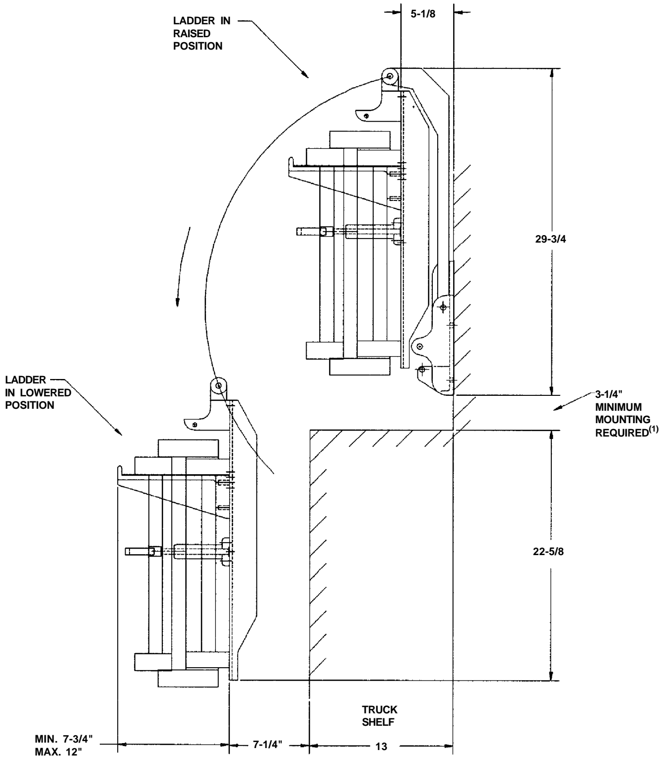
FIGURE 6. SIDE VIEW MODEL LAS-BHM-_____
