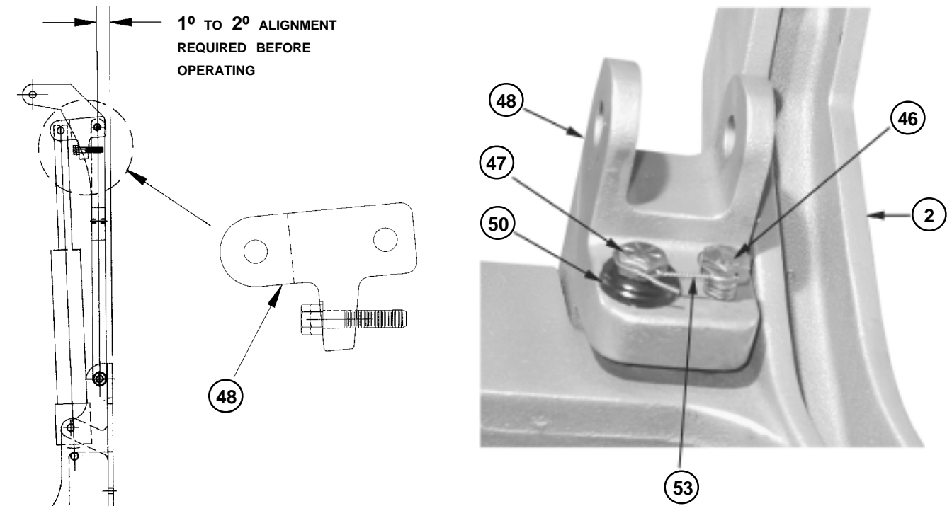
FIGURE 1 ACTUATOR RETAINER ADJUSTMENT (See Section VI. D. 1.)
