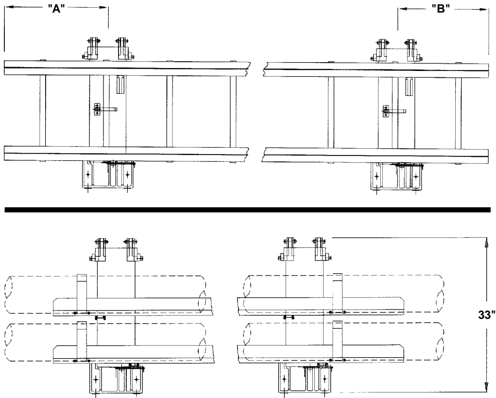
FIGURE 10. FRONTAL VIEW OF HSS SYSTEM
