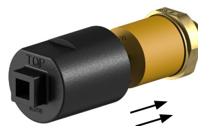
Figure 2: Sprinkler VK680 Installation and Correct Use of Wrench
