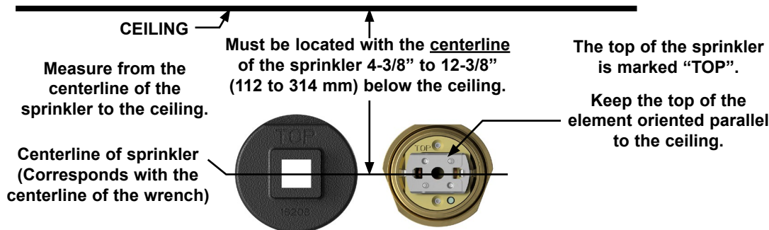
Figure 3: Sprinkler VK680 Correct Deflector Orientation
