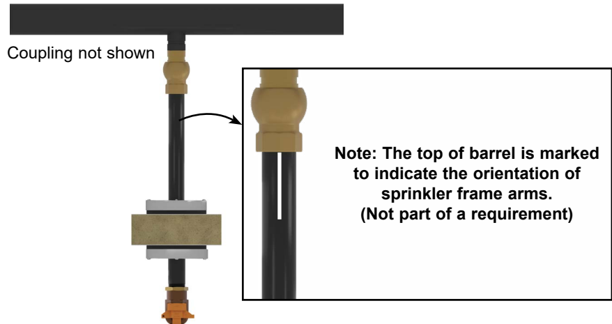
Figure 2: Sprinkler Installation
