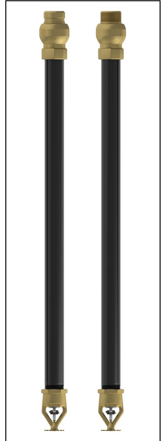
ESFR Sprinkler VK504 (Grooved and Threaded)
