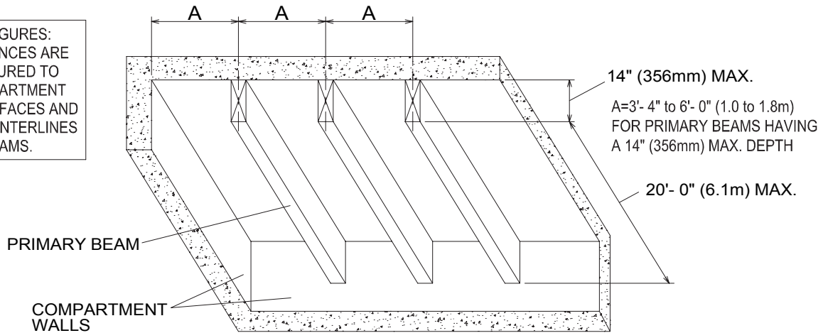
FIGURE 4A. PRIMARY BEAM SPANS UP TO 20'-0" (6.1m)
