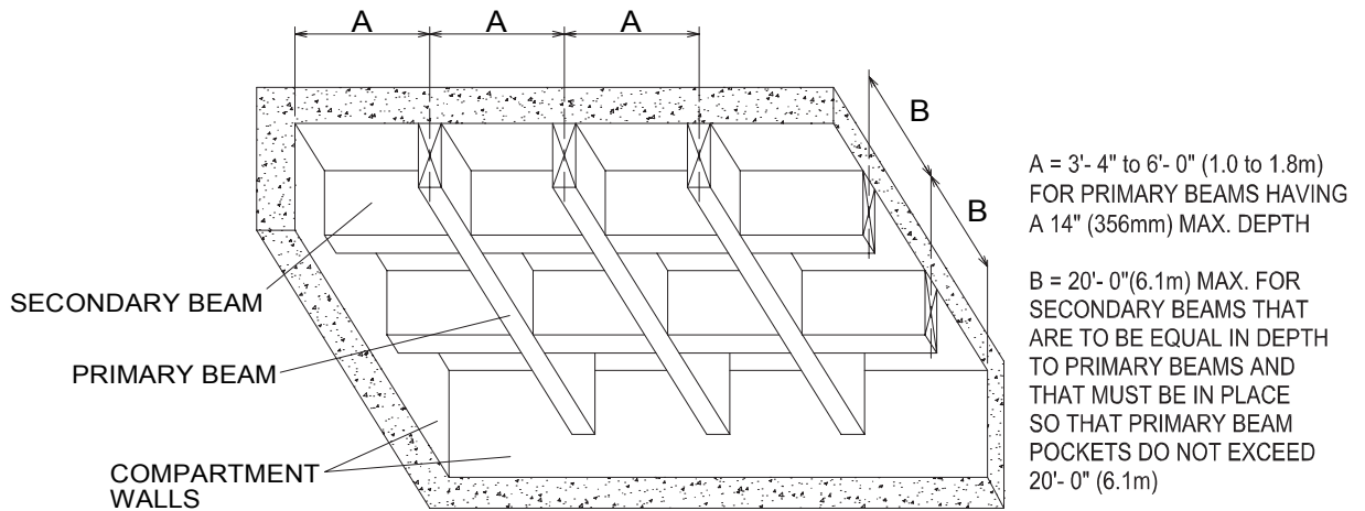
FIGURE 4B. PRIMARY BEAM SPANS GREATER THAN 20'-0" (6.1m)
