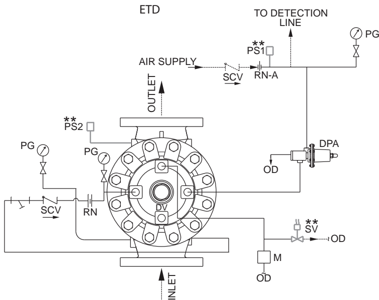
SCHEMATIC 2
