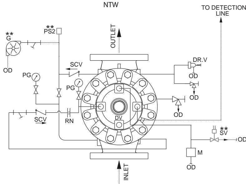
SCHEMATIC 7
