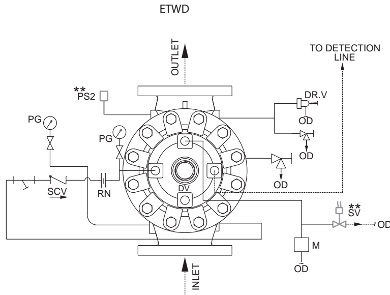
SCHEMATIC 5
