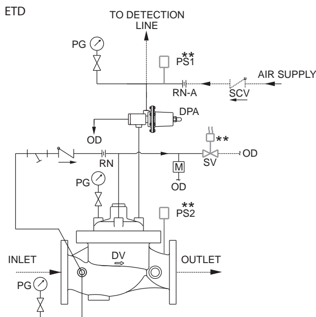
SCHMATIC 10
