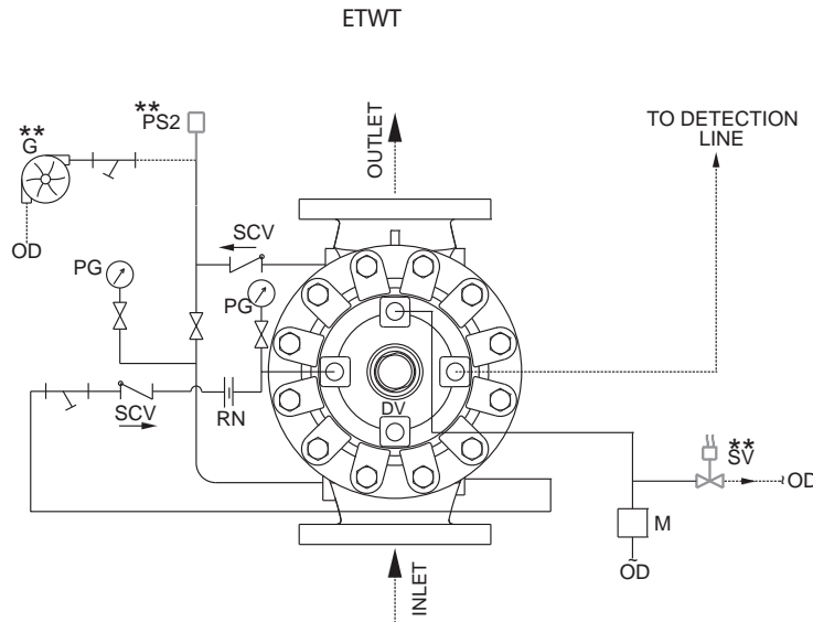
SCHEMATIC 3
