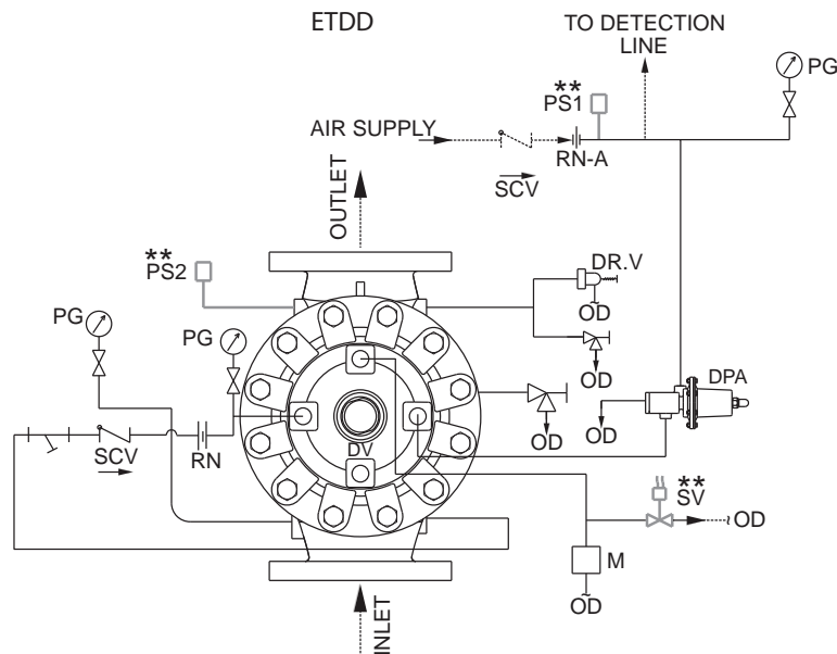
SCHEMATIC 6
