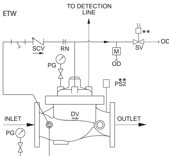
SCHMATIC 9
