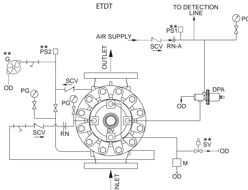
SCHEMATIC 4
