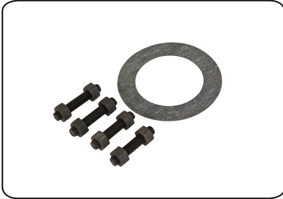
Nuts, Bolts and Gasket Package for mounting monitors onto an existing flange mount.
