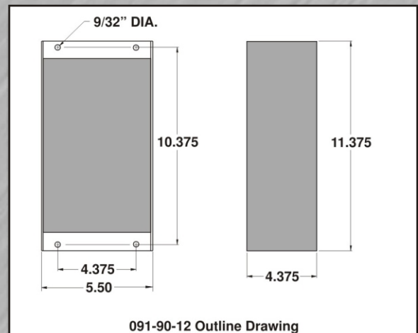
091-90-12 Outline Drawing
