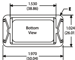
EURO and NGR Outline Drawing
