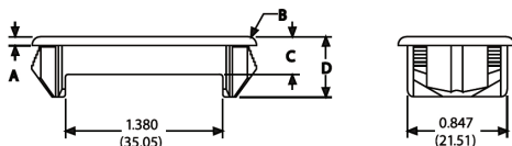
SVR Outline Drawing
