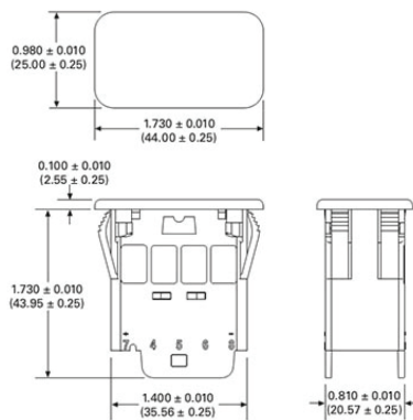
SVR Outline Drawing
