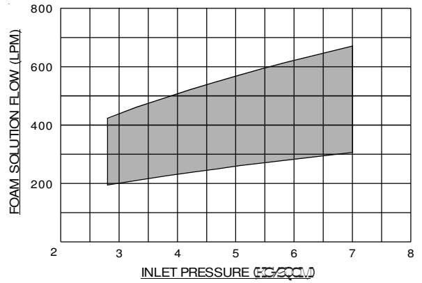
SIZE 65NB
