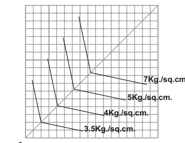
SPRAY AT 45° UPWARD
